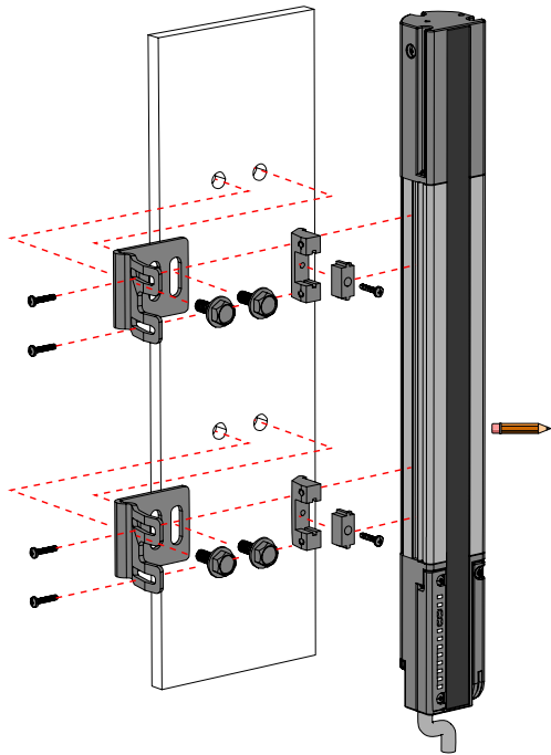
Figure 13. Side-Mount Brackets
