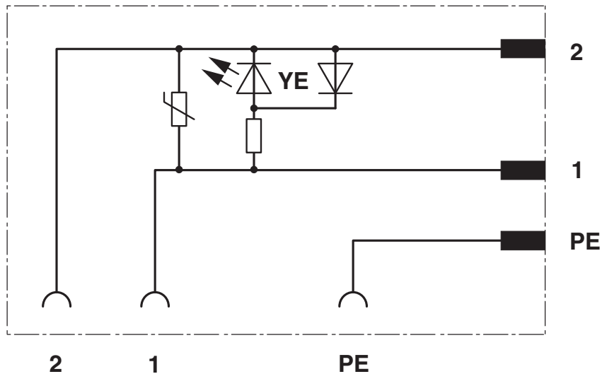
Circuit diagram
